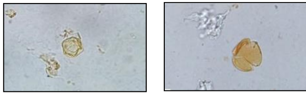
Gambar 5. Fossil Palinomorf Mangrove-Backmangrove : 1. Acrosthicum aureum (1000X), 2. Zonocostites ramonae (1000X), 3. Spinizonocolpites echinatus (1000X), 4. Discoidites borneensis (1000X), 5. Discoidites novaguensis (1000X), 6. Oncosperma type (1000X), 7. Acanthus type (1000X), 8. Aegialitis spp. (1000X), 9. Lumnitzera spp. (1000X), 10. Avicennia type (1000X)
