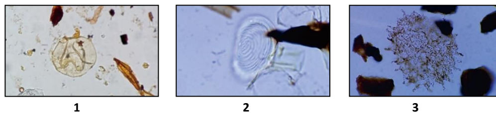
Gambar 8. Fossil Algae Freshwater : 1. Bosedinia type (1000X), 2. Concentricystes circula (1000X), 3. Pediastrum (1000X)
