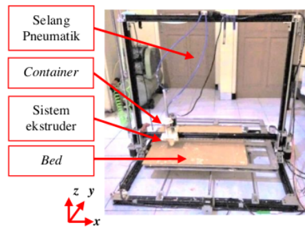
Gambar 1. Mesin 3D Printer FDM Customized
