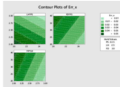
Gambar 6. Contour plots respon error dimensi x
