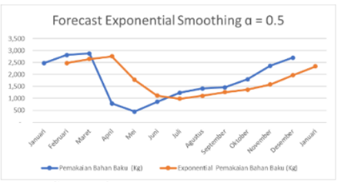
Gambar 4 Exponential Smoothing \alpha = 0.5
