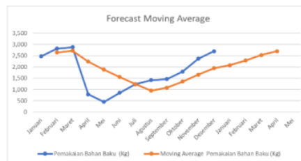
Gambar 2 Forecast Moving Average 2020
