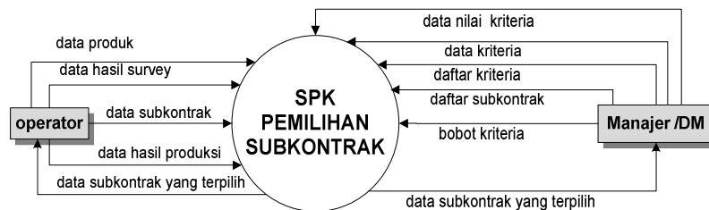
Gambar 2. Data Flow Diagram Level 0
