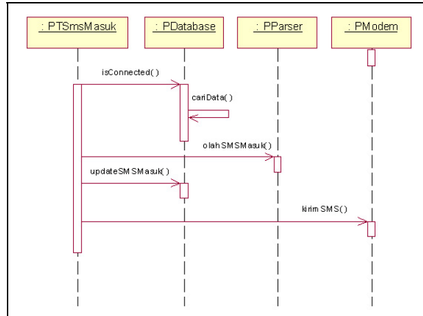
Gambar 6. Diagram Sequence Mengirim SMS Balasan
