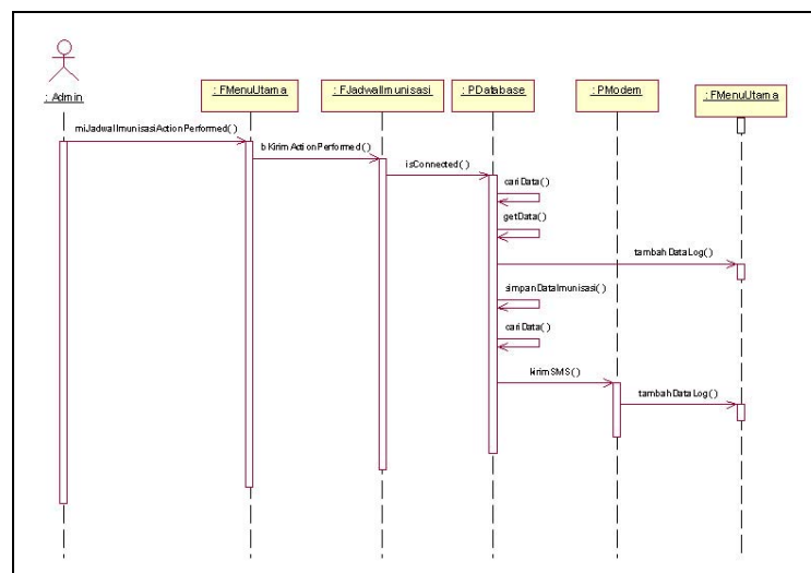
Gambar 8. Diagram Sequence Mengirim Jadwal Imunisasi
