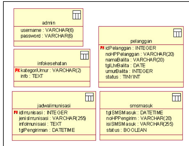
Gambar 10. Data Model Diagram
