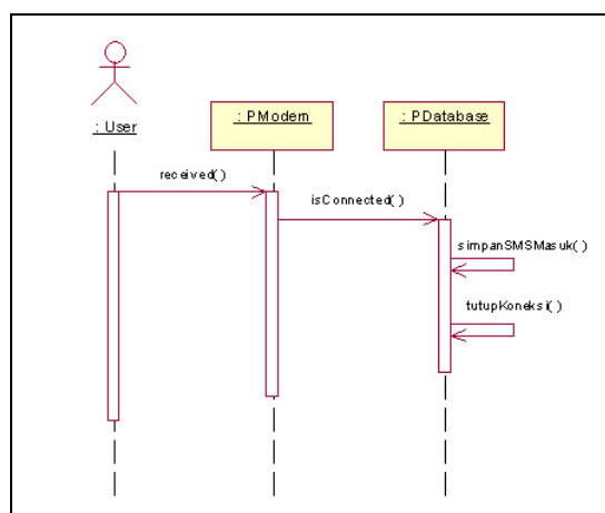
Gambar 5. Diagram Sequence Berhenti Berlangganan
