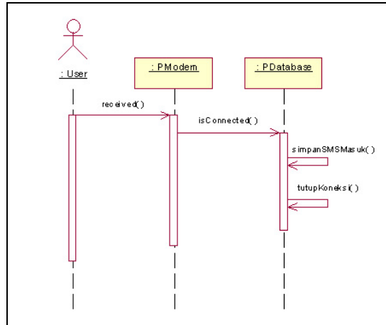
Gambar 3. Diagram Sequence Registrasi Berlangganan
