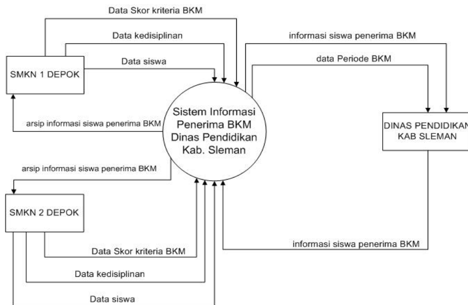
Gambar 1. DFD Level 0
