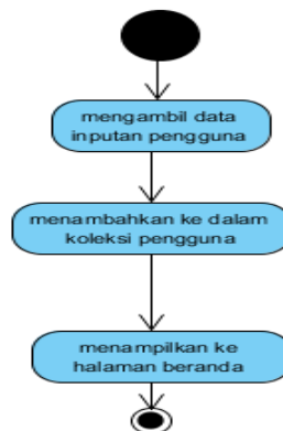
Gambar 3.3 Activity Diagram Fungsi input Buku
